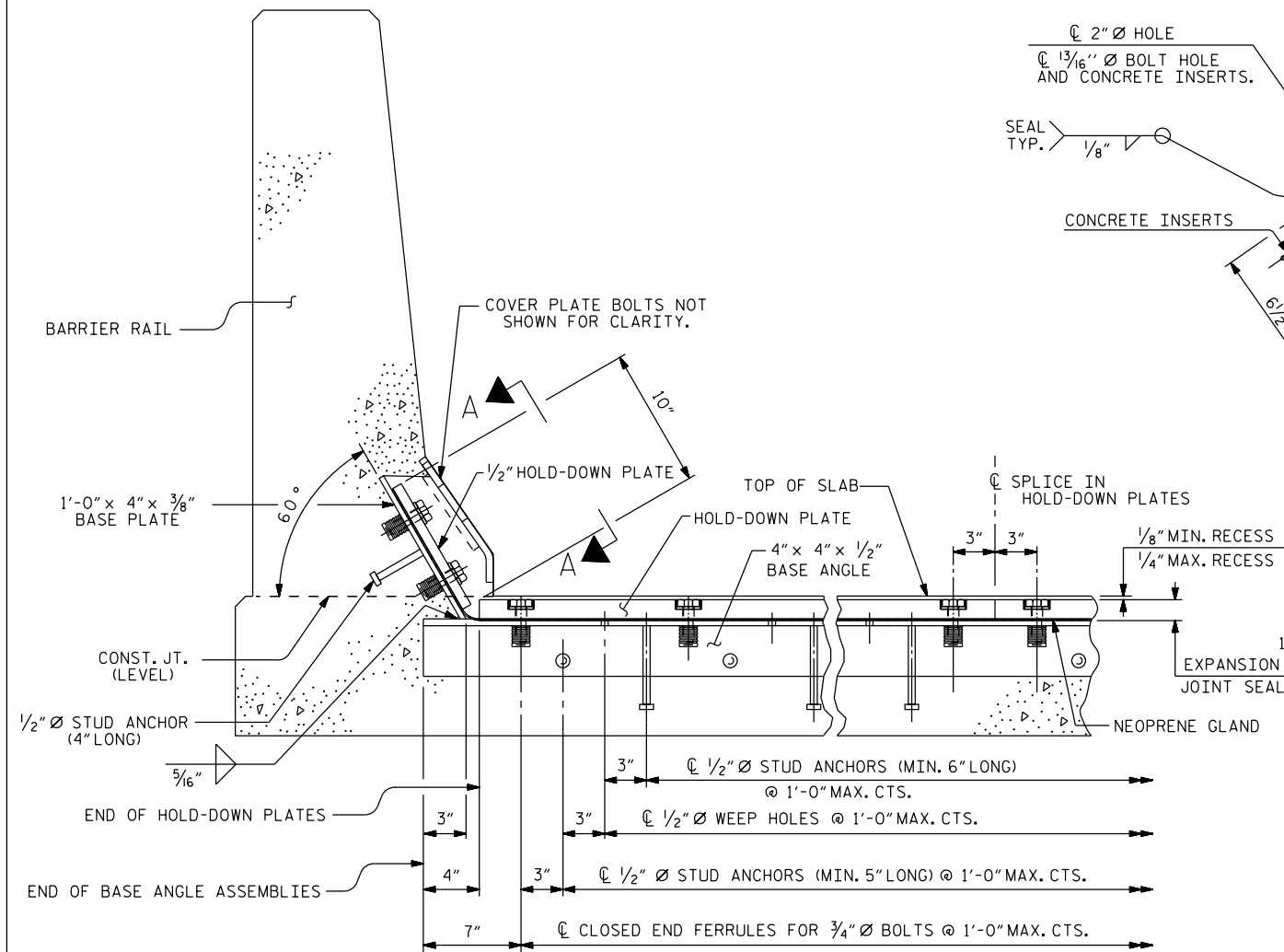
SECTION THRU RAIL NORMAL TO JOINT
