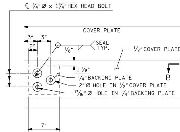
TYPE I - ELEVATION VIEW
