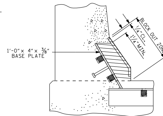
BLOCK OUT DETAIL
