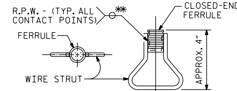
PLAN ELEVATION
