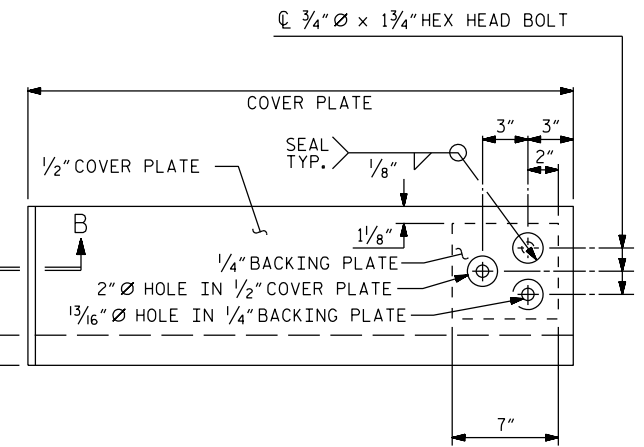
TYPE II - ELEVATION VIEW
